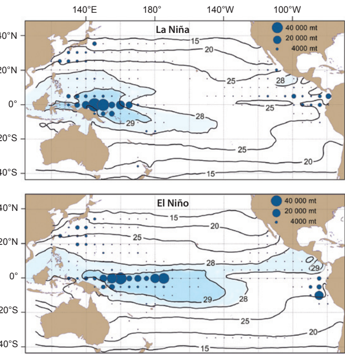
Figure 1 Representative skipjack tuna catches (blue circles) in the Western and Central Pacific Ocean during a La Niña event (top panel), and an El Niño event (bottom panel). Lines are isotherms (°C). Source: Lehodey et al. (2011) Chapter 8 PDF: http://www.spc.int/climate-change/fisheries/assessment/main-book.html
