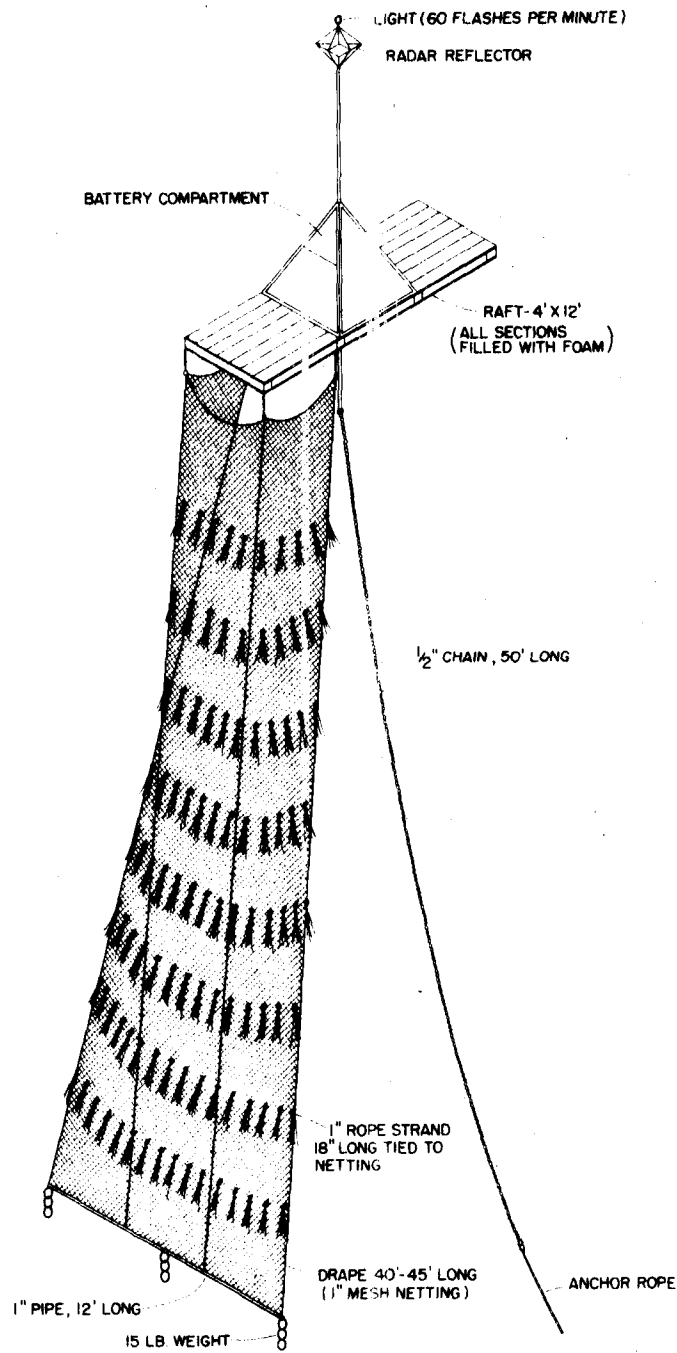
Figure 4.--Fish aggregating device, raft type.
